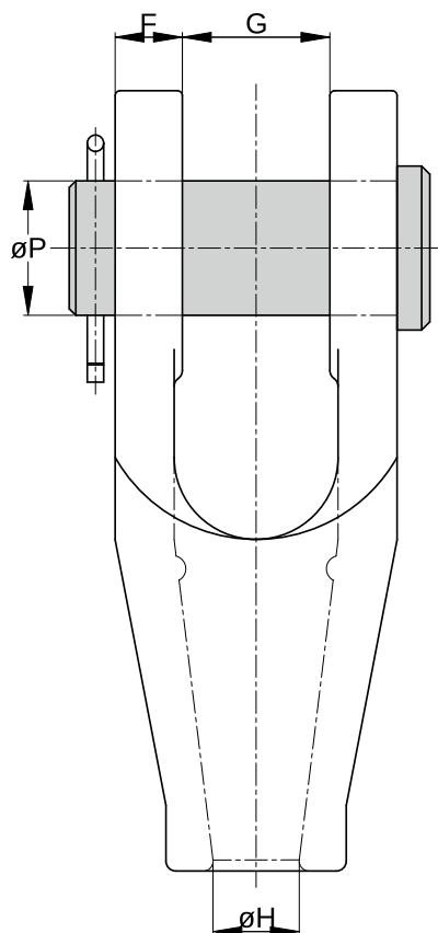
with pin
