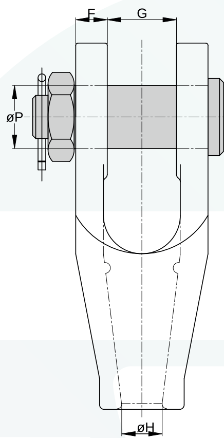
with bolt
